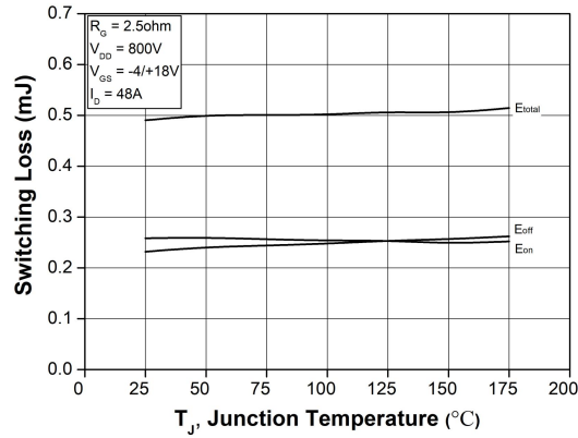
Figure 25. Clamped Inductive Switching Energy vs. Temperature
