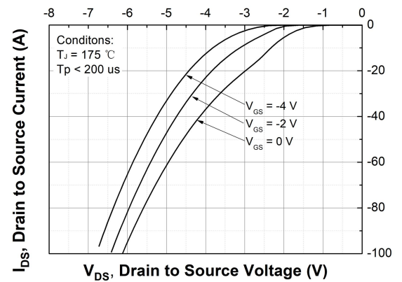
Figure 10. Body Diode Characteristic at T_J = 175 °C
